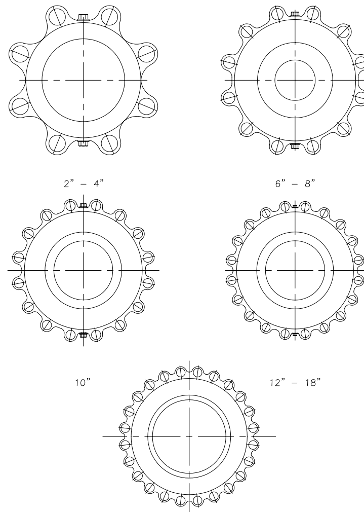
Hole Configuration
