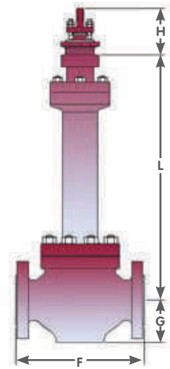
Valve with Bellows seal bonnet
