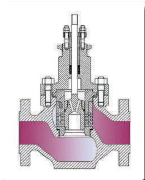
LR 2 Double Stage Low Pressure Recovery
