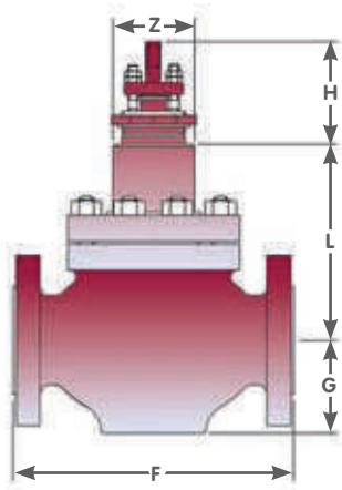
Valve with Standard bonnet
