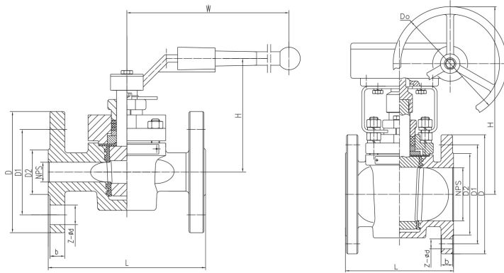
Main External and Connection Dimension
