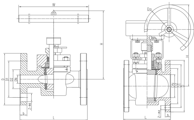
Main External and Connection Dimension
