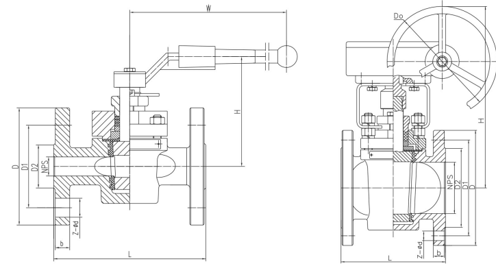
Main External and Connection Dimension
