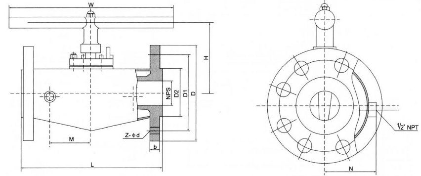
Main External and Connection Dimension
